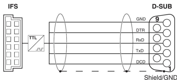
Figure 3 IFS-RS232-DATACABLE
